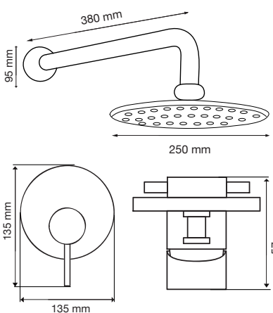
Kit Regadera New York Mod. 83.0103
