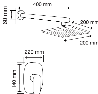
Kit Regadera Porto Mod. 84.0103
