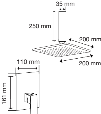
Kit Regadera Lexus a techo Mod. 75.0104C
