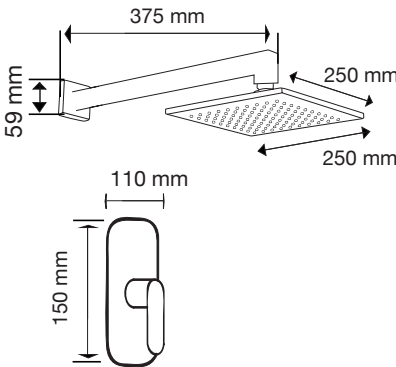
Kit Regadera Porto Mod. 84.0103
