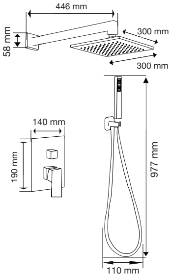
Kit Regadera Pisa Mod. 82.0105C
