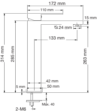
Monomando Alto Mod. 75.1129
