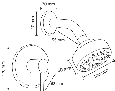
Kit Regadera Damasco Mod. 32.0103C
