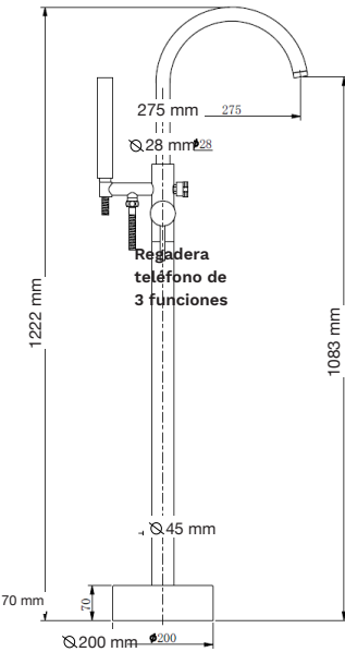
Monomando Bañera Victoria Mod. 8537
