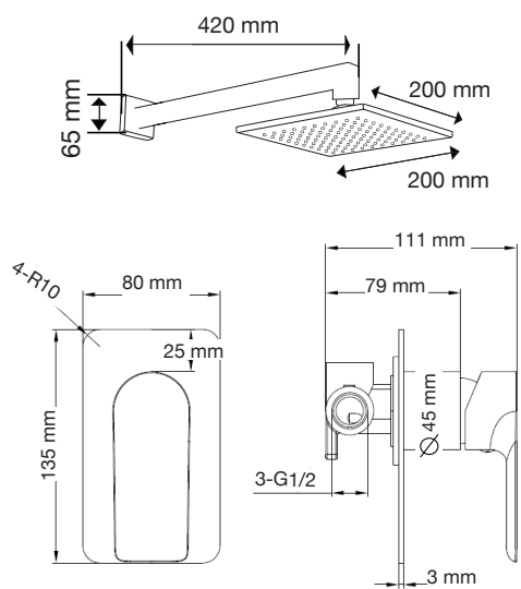
Kit Regadera Odessa Mod. 73.0103N
